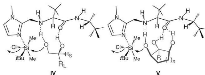
Scheme 2. Proposed models for enantioselective silylations in Tables 1 and 2.
